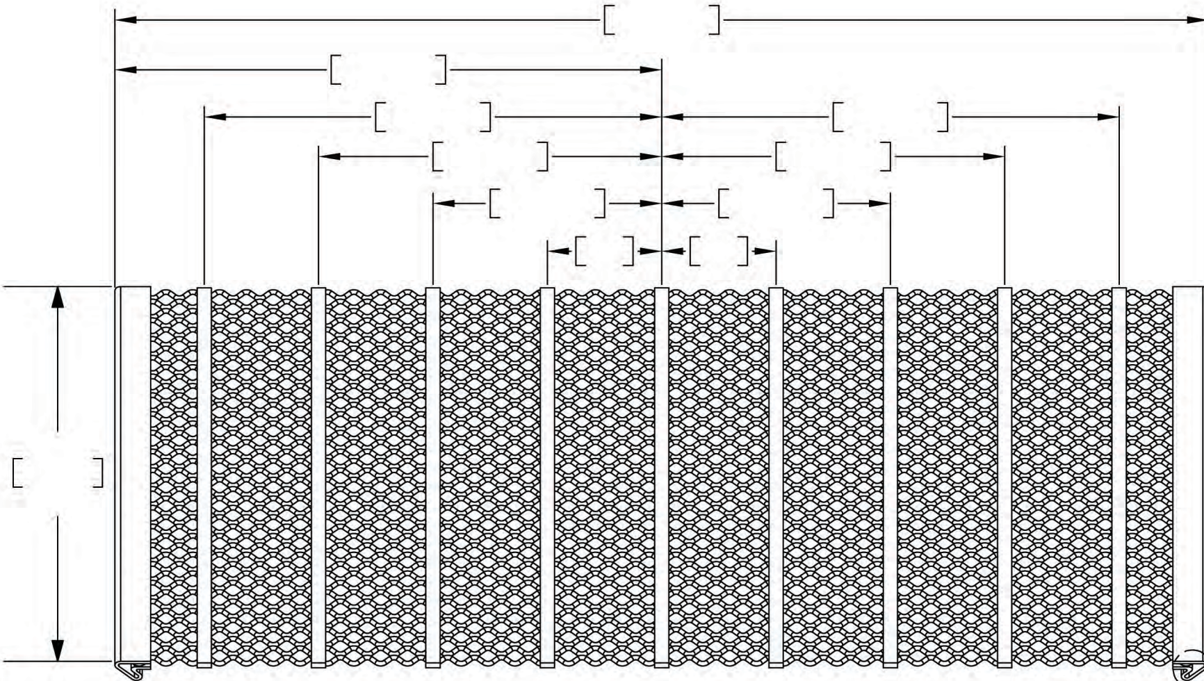
DETAIL A-A TYPE 5 HOOK
