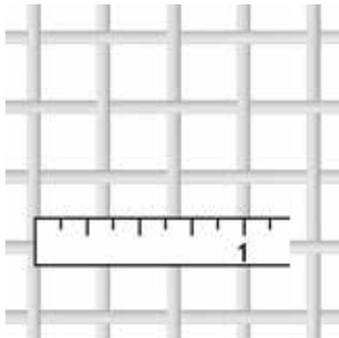
3 Mesh; .063" Wire 65.6% Open Area
